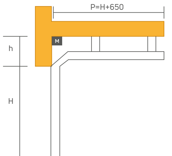
Architrave standard
