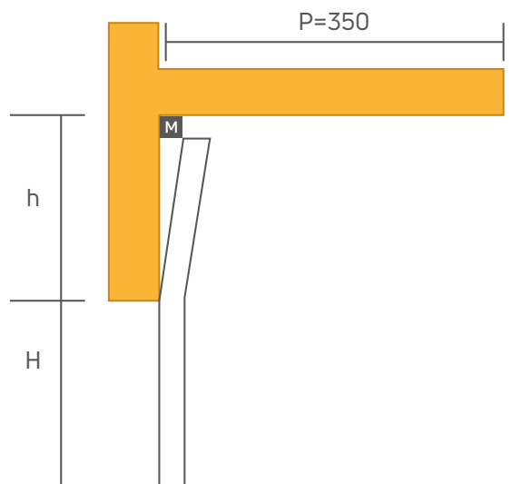
Architrave verticale
